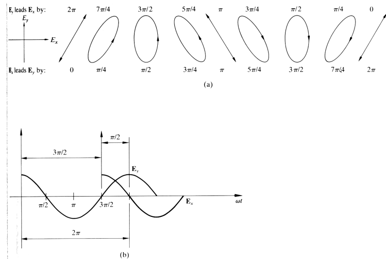
Figure 8.7 (a) Various polarization configurations. The light would be circular with \epsilon = \pi/2 or 3\pi/2 if E_{0x} = E_{0y} , but here for the sake of generality E_{0y} was taken to be larger than E_{0x} . (b) E_x leads E_y (or E_y lags E_x ) by \pi/2 , or alternatively, E_y leads E_x (or E_x lags E_y ) by 3\pi/2 .
