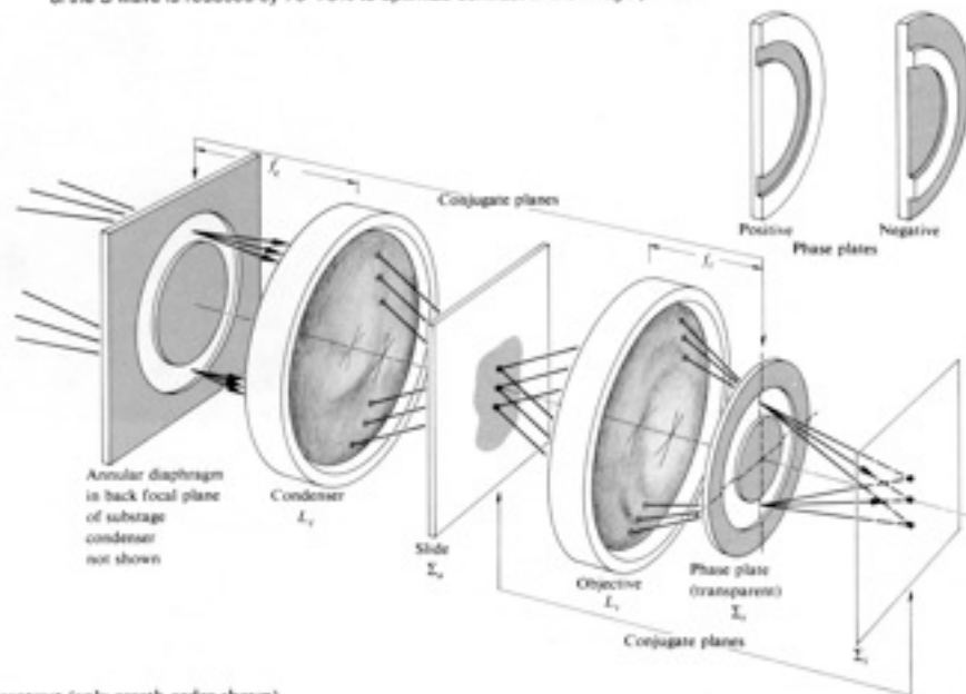
Figure 14.19 Phase contrast (only zeroth order shown).
