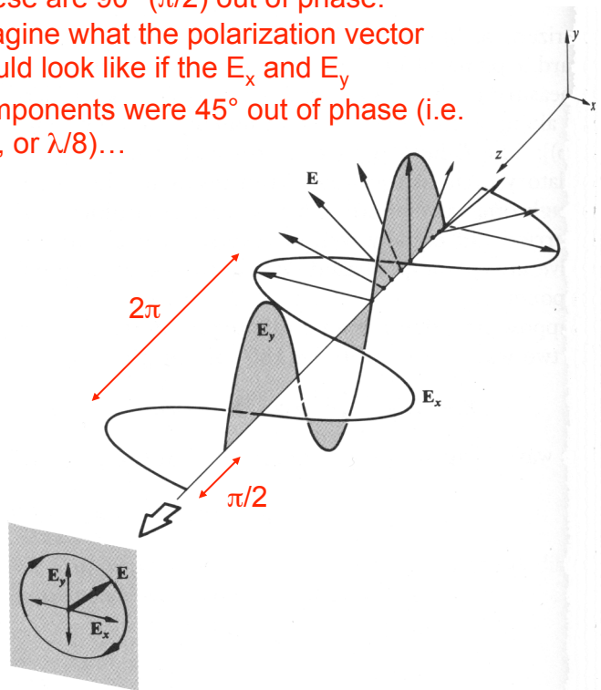
Figure 8.3 Right-circular light
