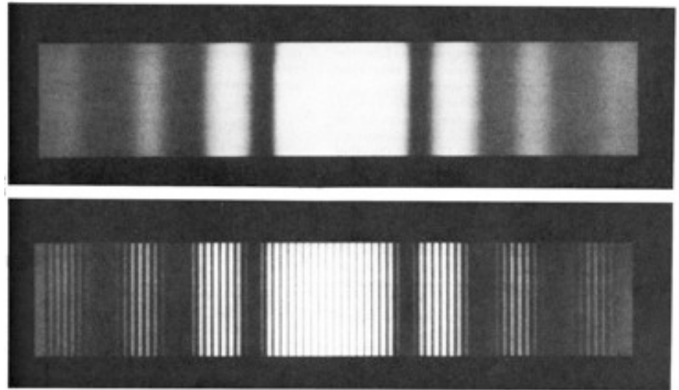
Figure 10.17 Single- and double-slit Fraunhofer patterns. The faint cross-hatching arises entirely in the printing process. (Photos courtesy M. Cagnet, M. Francon, and J. C. Thieffry: Atlas optique des diffractions , Berlin-Heidelberg-New York: Springer, 1962.)
