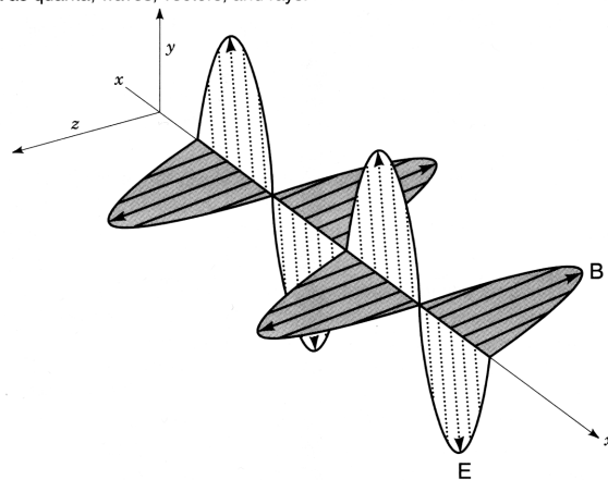
Figure 2-2 Light as an electromagnetic wave. The wave exhibits electric ( E ) and magnetic ( B ) fields whose amplitudes oscillate as a sine function over dimensions of space or time. The amplitudes of the electric and magnetic components at a particular instant or location are described as vectors that vibrate in two planes perpendicular to each other and perpendicular to the direction of propagation. However, at any given time or distance the E and B vectors are equal in amplitude and phase. For convenience it is common to show only the electric field vector ( E vector) of a wave in graphs and diagrams and not specify it as such.
