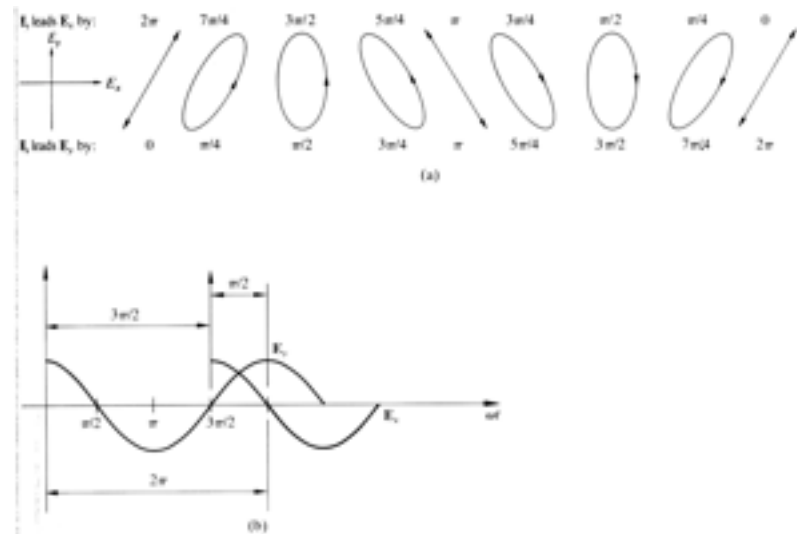
Figure 8.7 (a) Various polarization configurations. The light would be circular with \alpha = \pi/2 or 3\pi/2 if E_{0x} = E_{0y} , but here for the sake of generality E_{0x} was taken to be larger than E_{0y} . (b) E_x leads E_y (or E_y lags E_x ) by \pi/2 , or alternatively, E_x leads E_y (or E_y lags E_x ) by 3\pi/2 .
