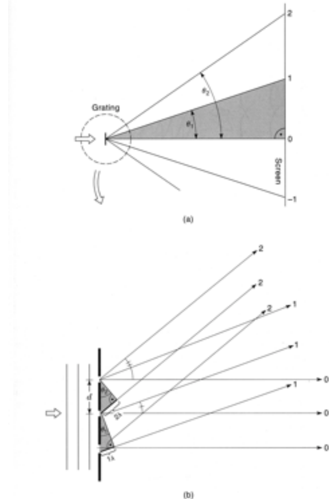
Figure 5-9 Dependence of scattering angle on grating spacing and wavelength. (a) Rays from a diffraction grating projected on a viewing screen. The angle of scattering of the 1 st - and 2 nd -order rays is shown as \theta_1 and \theta_2 . The grating and 1 st - and 2 nd -order spots define a right triangle that includes \theta_1 , and is congruent with a triangle that can be delineated at the grating as shown in (b). (b) The diffracted rays at the grating define a right triangle that includes diffraction angle \theta . For the 1 st - and 2 nd - etc.-order diffracted rays, the base of the triangle is an integral number of wavelengths, 1\lambda , 2\lambda etc. Thus, the angle of diffraction depends on two parameters: the grating spacing d and wavelength \lambda .
