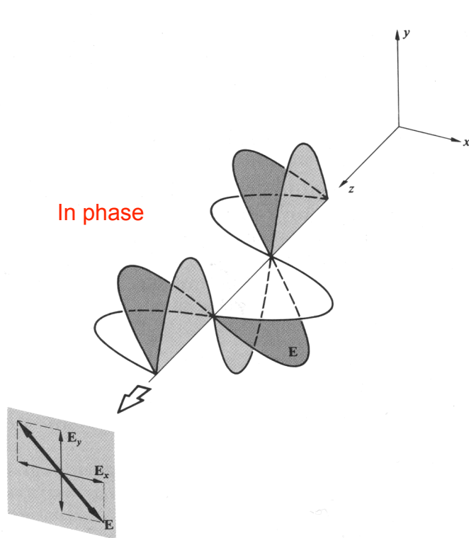
Figure 8.2 Linear light.
