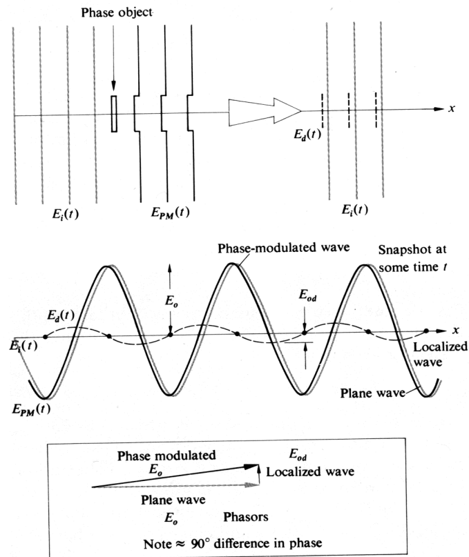
Figure 14.17 Wavefronts in the phase-contrast process.
