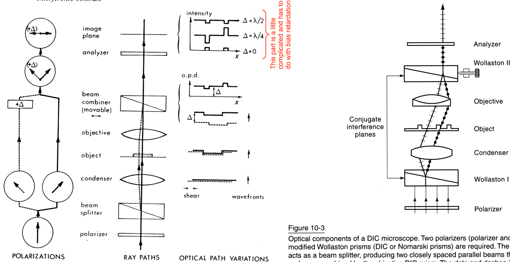
Fig. 38. The optical system for interference contrast.
