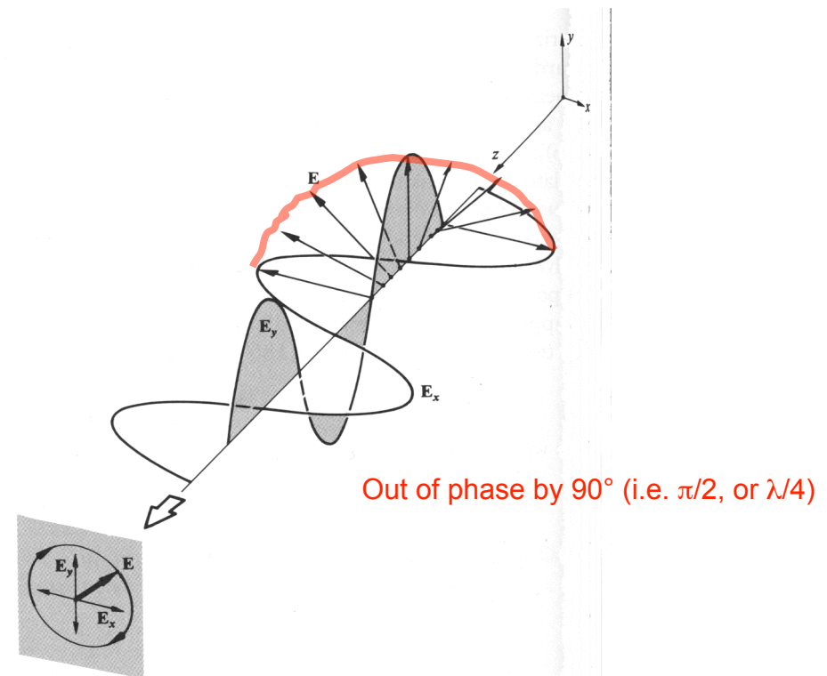
Figure 8.3 Right-circular light.
