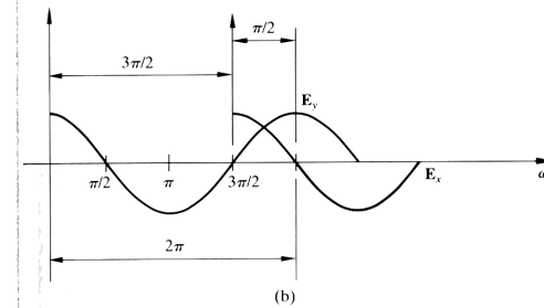
Figure 8.7 (a) Various polarization configurations. The light would be circular with \epsilon = \pi/2 or 3\pi/2 if E_{0x} = E_{0y} , but here for the sake of generality E_{0y} was taken to be larger than E_{0x} . (b) E_x leads E_y (or E_y lags E_x ) by \pi/2 , or alternatively, E_y leads E_x (or E_x lags E_y ) by 3\pi/2 .
