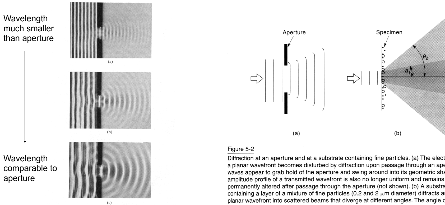
Figure 10.2 Diffraction through an aperture with varying \lambda as seen in a ripple tank. (Photo courtesy PSSC Physics, D. C. Heath, Boston, 1960.)
