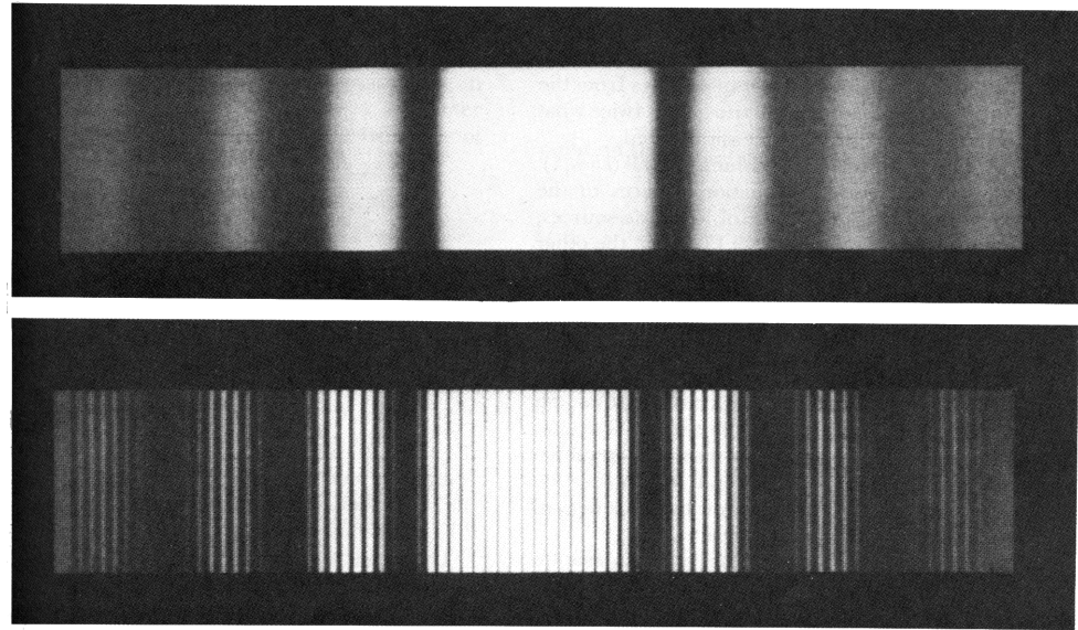
Figure 10.17 Single- and double-slit Fraunhofer patterns. The faint cross-hatching arises entirely in the printing process. (Photos courtesy M. Cagnet, M. Francon, and J. C. Thierr: Atlas optique des Erscheinungen , Berlin-Heidelberg-New York: Springer, 1962.)
